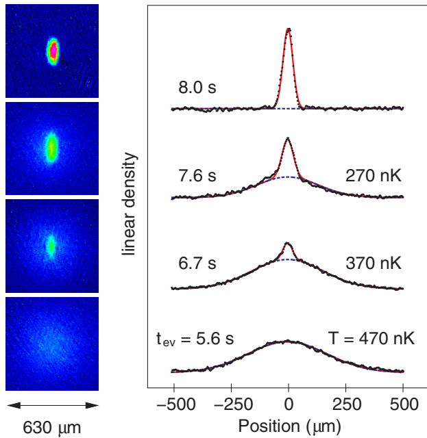
FIG. 2 (color online). Absorption images and integrated density profiles showing the BEC phase transition for different times t_{ev} of the evaporative cooling ramp. The images are along the vertical direction 25 ms after release from the trap. The solid line represents a fit with a bimodal distribution, while the dashed line shows the Gaussian-shaped thermal part, from which the given temperature values are derived.
