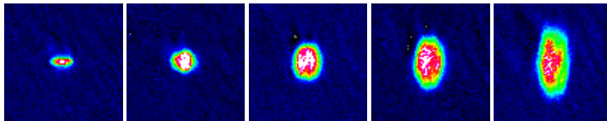
FIG. 3 (color online). Inversion of the aspect ratio during the expansion of a pure BEC. The images (field of view 250 \mu\text{m} \times 250 \mu\text{m} ) are taken along the vertical direction. The first image is an in situ image recorded at the time of release. The further images are taken 5, 10, 15, and 20 ms after release.
