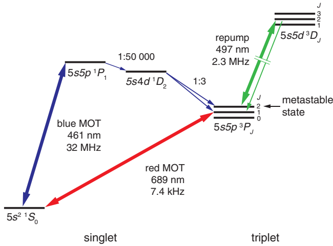
FIG. 1 (color online). Schematic illustration of the energy levels and transitions used for cooling and trapping of Sr atoms. The blue MOT is operated on the strong ^1S_0 - ^1P_1 transition. The loading of the magnetic trap proceeds via the weak leak of the excited state (branching ratio 1:50 000) into the ^1D_2 state, which itself decays with a 1:3 probability into the metastable ^3P_2 state. Here the atoms can be magnetically trapped and accumulated for a long time. The transition ^3P_2 - ^3D_2 allows us to depopulate the metastable state by transferring the atoms into the ^3P_1 state. The latter represents the excited state of the ^1S_0 - ^3P_1 intercombination line, used for narrowline cooling in the red MOT.
