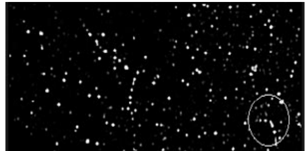
VIDEO 1: Observations of reconnecting quantized vortices captured by Paoletti et al. [1]. The movie is played in real-time (20 fps) and is 5.76 mm wide and 2.30 mm tall. The individual reconnection events are annotated by white circles and evidenced by groups of hydrogen clusters rapidly separating from one another. The clusters that are trapped on the vortices enable the authors to measure the separation as the vortices approach and retract from one another. (M. S. Paoletti et al. [1]) Video available at: http://physics.aps.org/articles/v1/26#video .
