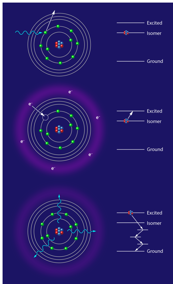
FIG. 1: This graphic shows the secondary process by which XFEL light can drive the energy release from a sample containing a nuclear isomer. In the first step (top), photons knock electrons out of inner atomic shells, leading to a plasma of free electrons and ionized atoms. This interaction does not directly affect the nucleus, as it remains in the metastable isomeric state (top right). However, when electrons from the plasma are later captured in the inner-shell vacancies, their excess energy can excite the nucleus to a higher, but less stable, energy state (middle). In the last step, the nucleus relaxes to its ground state, releasing photons in a cascade (bottom). (APS/Alan Stonebraker)
