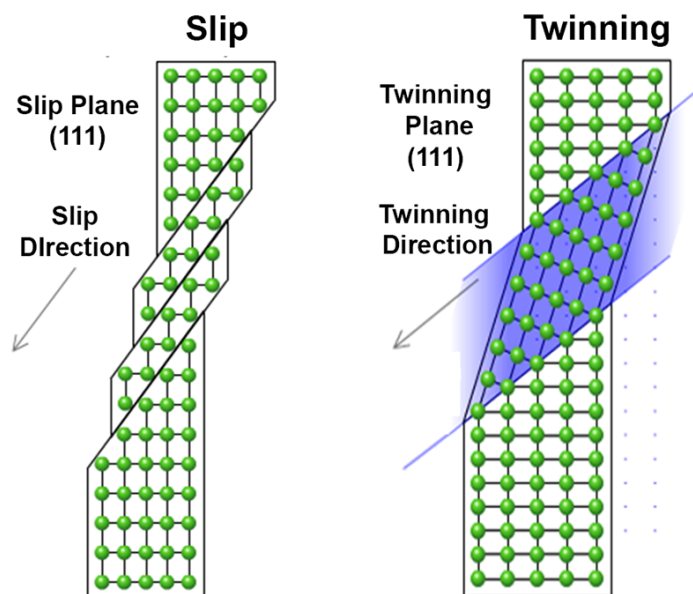
Figure 2: Cartoon of slip and twinning deformations in a face-centered cubic crystal. (Left) Slip occurs when dislocations glide through the material, causing crystal planes to slide along each other. (Right) Twinning occurs via a concerted shift of atomic positions in the twinning direction. The twin crystal's structure is a mirror image of the parent structure about the twinning plane. (DoITPoMS/University of Cambridge)
