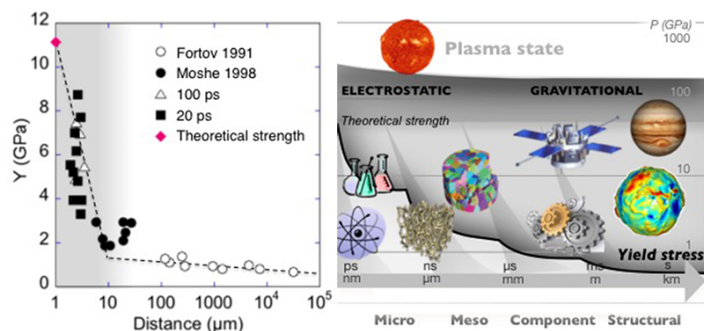
Figure 1: (Left) Tensile strength of pure aluminum as a function of the dimensions of the loaded material. (Right) Variation of yield stress observed in condensed matter at different scales, from atomic scales, where electrostatic effects dominate, to planetary scales, where the yield stress sinks to zero and gravitational forces prevail. (Neil K. Bourne/University of Manchester; Image on homepage: F. Zhao et al. [1])
