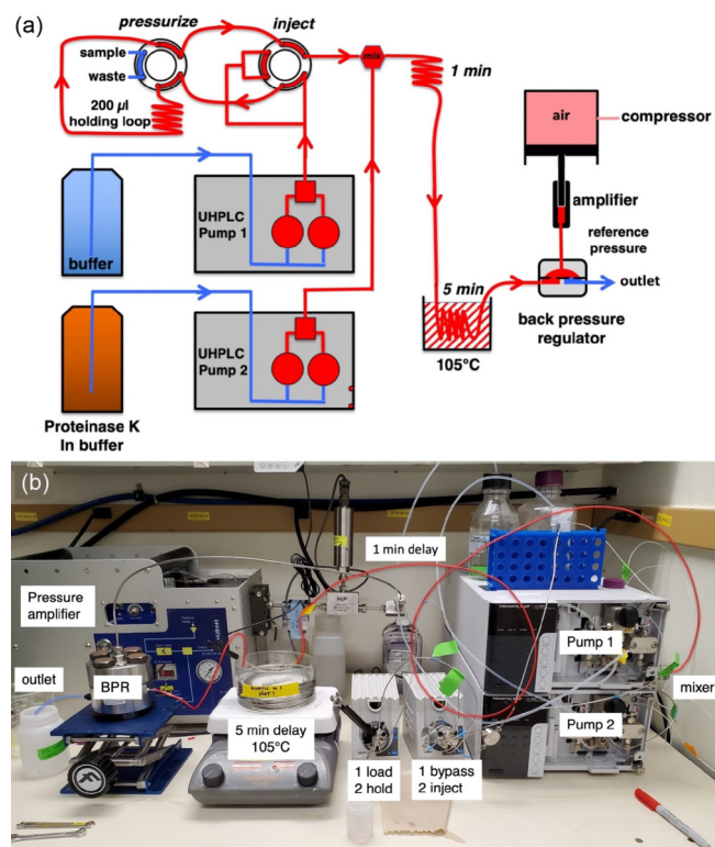
FIG. 2. Apparatus to perform Hi-P LiP. (a) Schematic of apparatus that can perform precisely timed pulse proteolysis of cellular extracts under high pressure followed by thermal denaturation and recovery. Blue lines represent fluid supplied at ambient pressure; red lines are fluid under pressure. (b) Photograph of apparatus in operando . BPR, back-pressure regulator. The two six-port valves shown, each with setting 1 or 2, define the sample injection complex (see Figs. S1(a)–S1(c) in the SM [23]).
