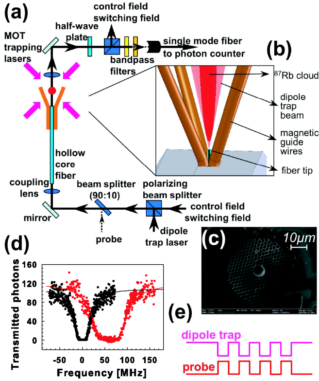
FIG. 1 (color online). (a) Schematic of the experimental setup. (b) Schematic detail of the fiber loading. Inside the fiber, the atoms are transversely trapped by an optical trap formed by a single beam guided by the fiber. After exiting the top end of the fiber the divergent beam creates a funnel potential guiding the atoms into the fiber core from a distance up to \sim 100 \mu\text{m} . The atomic cloud is moved into this region by a magnetic guide consisting of four current-carrying wires that fan out from the fiber tip. (c) Scanning electron microscope image of the fiber cross section. The diameter of the central hollow region is 7 \mu\text{m} . (d) Transmission through the fiber loaded with \sim 3000 atoms as a function of probe detuning from the (5S_{1/2}, F=1) \rightarrow (5P_{1/2}, F'=2) transition. Red points show the absorption profile with the dipole trap on continuously. Comparison to the calculated profile based on the dipole trap parameters (solid red line) confirms that the atoms are loaded inside the fiber. Black points show the observed absorption profile when probe and dipole trap are modulated as shown in (e). Here, a homogeneous broadening is caused solely by the large optical depth of the system.
