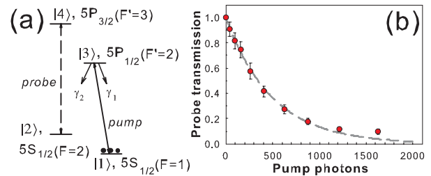
FIG. 2 (color online). (a) Four-state atomic system for nonlinear saturation based on incoherent population transfer. (b) Transmission of the probe as a function of the number of incident pump photons with exponential fit. 50% reduction of probe transmission is achieved with \sim 300 pump photons.
