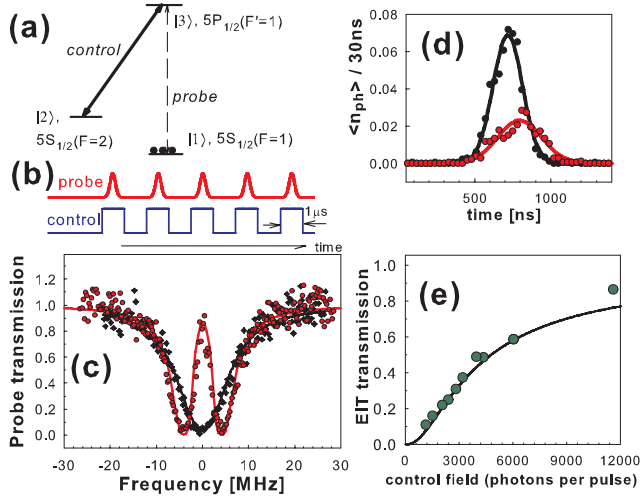
FIG. 3 (color online). (a) Three-level \Lambda -scheme used for EIT in the mesoscopic atomic medium. (b) Both probe and control field are broken into a set of \sim 100 synchronized pulses sent through the fiber during the off-times of the dipole trap. The probe pulses have Gaussian envelopes with rms width t_p \sim 150 ns. (c) Probe transmission through the fiber without (black data points) and with (red data points) control field (each data point corresponds to 100 individual pulses). Solid lines are fits of Eq. (2). (d) Individual probe pulse shape and delay. The EIT pulse (red) is delayed by \sim 100 ns compared to the reference pulse (black), for control pulses containing \sim 3500 photons. Data points represent the average number of photons detected in a 30 ns time bin. (e) Observed transmission of the probe pulses on resonance as a function of average number of photons in the 1 \mu\text{s} control field pulse and the prediction (gray line) based on Eq. (2).
