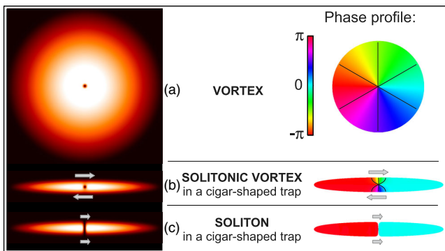
FIG. 2 (color online). Theoretical solutions of in situ density and phase profiles for (a) a vortex aligned along the axis of an axially symmetric potential, a solitonic vortex (b) and a soliton (c) oriented perpendicularly to the axis of an elongated axially symmetric trap. Arrows indicate the atomic flow.
