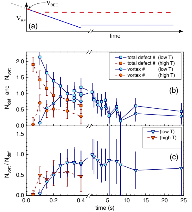
FIG. 4 (color online). (a) Sketch of the evaporation ramp. (b) Number of total defects (squares) and of solitonic vortices (dotted circles) measured on average at different times during and after the evaporation ramp. Blue (solid) and red (dashed) points correspond to data sets with different final evaporation frequencies. Error bars are evaluated as \sqrt{\sigma^2 + 1/N_m} , where \sigma is the standard deviation of the average counts and N_m the number of measurements. (c) Ratio between averaged counted solitonic vortices and total defects.
