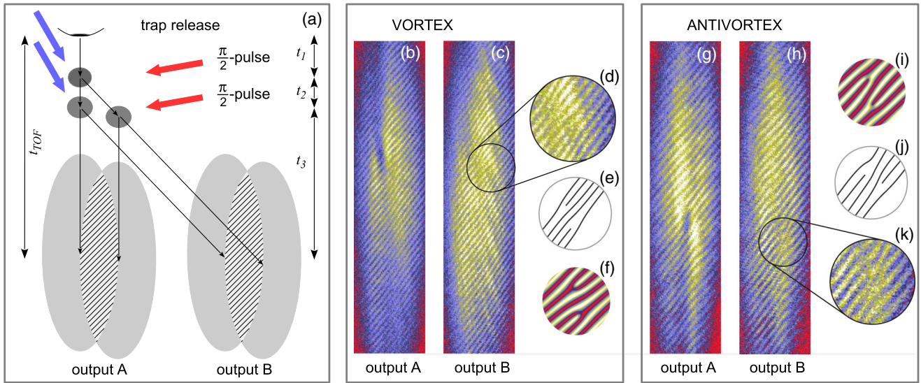
FIG. 3 (color online). (a) Time sequence for the two-pulse Bragg interferometer. After t_1 from the atoms release a first \pi/2 Bragg pulse splits the condensate in two parts, one at rest and the other moving at the Bragg velocity. After t_2 a second pulse further splits each condensate and imaging after a long t_3 allows for the separation of the two outputs and for the creation of the interference pattern. (b)–(c) Experimental images of the two interferometer outputs in the presence of a vortex with clockwise circulation. (d) Enlargement on the interference pattern showing the dislocation-antidislocation pair and a guide to the eye (e) sketching the interference pattern. (f) 2D numerical simulation of the experiment. (g)–(k) The same, but for an antivortex with counterclockwise circulation.
