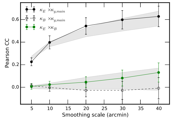
FIG. 3 (color online). The Pearson correlation coefficient between the foreground galaxy and convergence maps is shown as a function of smoothing scale. The solid and open symbols show correlation coefficients from the E and B modes of the convergence, respectively. The grey shaded regions show the 1\sigma bounds from simulations for the correlation between the E - and B -mode convergence and the foreground galaxies, with the same pixelization and smoothing as the data as well as sources of statistical uncertainty. The green points show the correlation between E and B modes of the convergence map. The various correlation coefficients with the B -mode convergence are consistent with zero. Uncertainties on all measurements are estimated using jackknife resampling.
