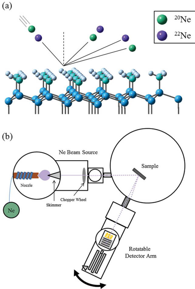
FIG. 1. (a) Illustration of a monoenergetic beam of 20 Ne and 22 Ne diffracting from CH 3 -Si(111) into spatially well-separated final scattering angles; (b) schematic of the ultrahigh vacuum surface scattering instrument employed in this experiment; key components are a high-Mach number, triply differentially pumped molecular beam source with variable temperature nozzle, a UHV scattering chamber with a full suite of diagnostics (not shown), and a high sensitivity triply differentially pumped detector with a high degree of collimation that can rotate to detect a range of final scattering angles while maintaining constant incident kinematic conditions.
