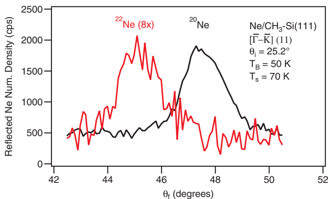
FIG. 3. Nearly complete angular separation of (11) diffraction peaks for ^{20}\text{Ne} (black) and ^{22}\text{Ne} (red) diffracted from \text{CH}_3\text{-Si}(111) . Further purification of the major ^{20}\text{Ne} component or separation and enrichment of the minor ^{22}\text{Ne} component can be realized through experimental considerations as discussed in the text.
