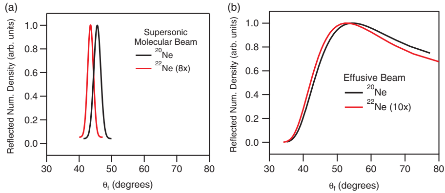
FIG. 2. (a) Demonstration of angular separation for supersonic molecular beam diffraction from an ideal grating for the conditions reported herein; (b) lack of angular separation for an effusive source under identical incident conditions; T_B = 55 K, \theta_i = 25.2^\circ .
