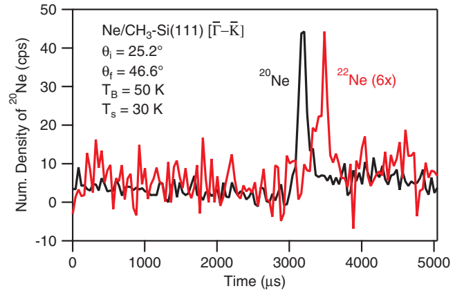
FIG. 5. Time-of-flight spectra for ^{20}\text{Ne} (black) and ^{22}\text{Ne} (red) at the midpoint between the maxima of the ^{20}\text{Ne} and ^{22}\text{Ne} (11) diffraction peaks as shown in Fig. 3, providing a route for temporal separation of the isotopes.
