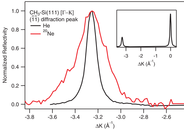
FIG. 4. (\bar{1}\bar{1}) diffraction peak for helium (black) and ^{20}\text{Ne} (red) scattering from \text{CH}_3\text{-Si}(111) . Note that the width of these peaks is a consequence of the convolution of the instrument function, surface quality, and their incident velocity distributions. The He diffraction peak has a significantly narrower angular distribution than the Ne peak, due to the narrower velocity distribution of the He beam used ( \Delta v/v = 0.8\% ) as compared to that for the Ne beam ( \Delta v/v = 6.4\% ). Potential further improvement in angular separation, as compared to the data shown in Fig. 3, can be realized by additional narrowing of the beam's incident velocity distribution. Inset: wide angular range diffraction scan for He/ \text{CH}_3\text{-Si}(111) , demonstrating the high quality of the substrate used in these experiments.
