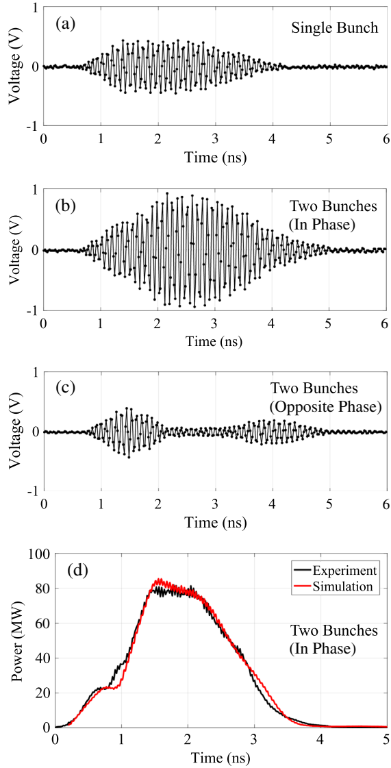
FIG. 6. Experimental measurements of backward power with two bunches. Voltage signal from (a) a single bunch, (b) two bunches with 0 deg phase difference, (c) two bunches with 180 deg phase difference. (d) Highest rf power from two bunches in phase with a total charge of 85 nC in perfect agreement with the CST PIC simulation.
