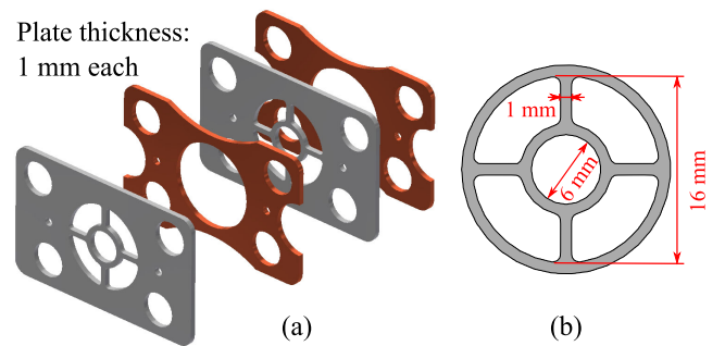
FIG. 2. MTM structure design. (a) Alternating wagon wheel plates and spacer plates. Forty plates of each type are clamped together to form an 8 cm long structure. (b) Wagon wheel plate geometry.
