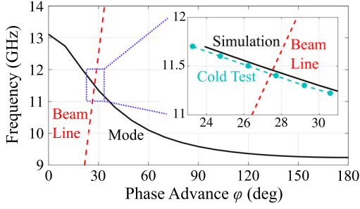
FIG. 3. Dispersion curve of the fundamental transverse magnetic mode intersecting with the beam line \omega = k_z v_z at 11.42 GHz, where k_z is the longitudinal wave number, and v_z is the beam longitudinal velocity. The horizontal axis represents the phase advance per period as \phi = k_z p , where p = 2 mm is the period. A bead pull measurement was done around the design frequency, as shown in the blow-up figure along with the simulation result.
