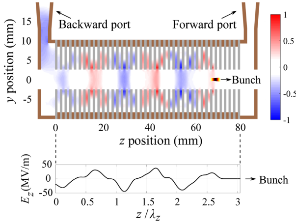
FIG. 4. Plot of the longitudinal electric field E_z . The two-dimensional field plot on the top shows the normalized E_z field on the middle plane in the linear scale. The MTM structure is represented in grey. The one-dimensional plot on the bottom shows the E_z field on the beam axis for a single 45 nC bunch. The distance is normalized to the longitudinal wavelength \lambda_z . In both figures, the electron bunch travels to the right. The peak accelerating field available to a trailing bunch (in the blue region) is 43 MV/m.
