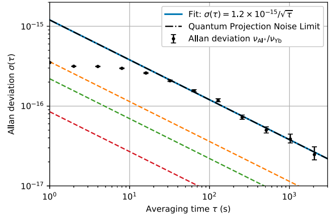
FIG. 4. Allan deviation of the frequency ratio \nu_{\text{Al}^+}/\nu_{\text{Yb}} measured over \approx 23000 s. The asymptote is fit to extract a frequency stability of \sigma(\tau) = 1.2 \times 10^{-15}/\sqrt{\tau} , where \tau is the averaging time in seconds. Anticipated stabilities for a correlation spectroscopy comparison of two single-ion ^{27}\text{Al}^+ clocks [37] (orange), a single ^{27}\text{Al}^+ mixed-species correlation comparison [38] (green), and a single ^{27}\text{Al}^+ ion clock operated using Rabi spectroscopy at the interrogation time of 20.6 s, equal to the excited state lifetime (red) are also shown.
