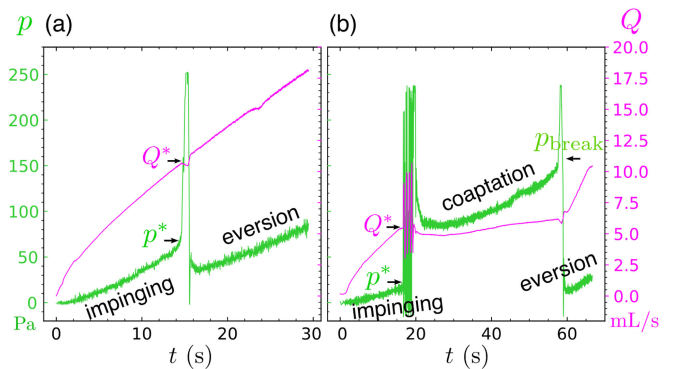
FIG. 6. Time sequence of the pressure p - t (green) and the flow rate Q - t (magenta) for (a) a steadily increasing flow past a conical shell, and (b) a flow with a short noise burst at \approx 18 s, collapsing it at much smaller p^* and Q^* .
