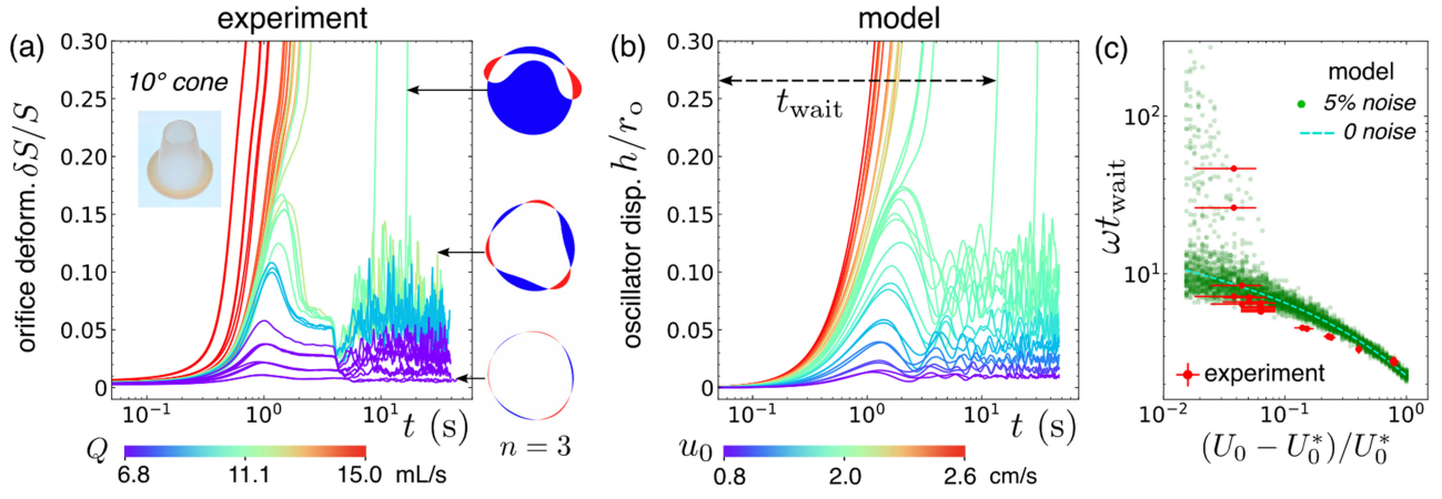
FIG. 4. Comparing experiment and theory for the flow-induced coaptation transition for a cone of \alpha = 10^\circ . (a) Measured orifice deformation, \delta S/S , under various flow rates (color bar). (b) Time evolution of the displacement x \equiv h/r_o from Eq. (3) (see SM [14] for parameter values) at various flow velocities (color bar). t_{\text{wait}} : the waiting time for the oscillator to diverge. (c) The normalized waiting time, \omega t_{\text{wait}} , for the cone to buckle (red markers, \omega = 2.66 ) and for the model oscillator to diverge (green dots, 5% noise), all plotted as a function of the normalized distance to the threshold, (U_0 - U_0^*)/U_0^* . Cyan dashed curve: the waiting time given by the model with no flow noise.
