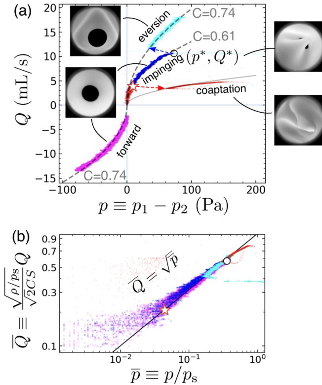
FIG. 3. The pressure-flow ( p - Q ) relation for a flow passing a conical shell of \alpha = 20^\circ . (a) The flow rate ( Q ) as a function of the pressure drop ( p ), for the flow along (magenta) or against (blue) the direction of narrowing of the cone. At (p^*, Q^*) (black open circle), the system buckles abruptly into an everted state (cyan). Injected flow noise causes an early buckling transition (red open star), resulting in a coaptation branch (red). Photographs: corresponding orifice shape for each branch. Dashed and solid curves: predictions from Eq. (1). (b) Rescaled pressure-flow relation, \bar{Q} - \bar{p} , collapsing all branches. Solid line: \bar{Q} = \sqrt{\bar{p}} .
