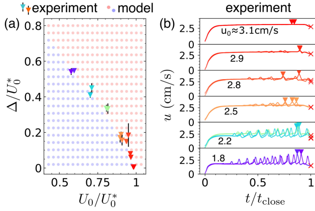
FIG. 5. Controlling closure with disturbances. (a) The disturbance amplitude \Delta required to trigger a transition ( \alpha = 20^\circ ) as a function of base flow U_0 , both normalized by the threshold velocity at zero disturbance U_0^* . Blue (red) dots: converging (diverging) solutions given by Eq. (3) at \tau \rightarrow \infty . (b) Experimental sequences of noise spikes of increasing amplitudes are injected to various base flows ( u_0 ) until the cone collapses (red crosses) at t_{\text{close}} . Multiple trials are shown for each base velocity, u_0 . Triangular markers in (a) and (b): measured minimal disturbance required to collapse the cone at various impinging flows.
