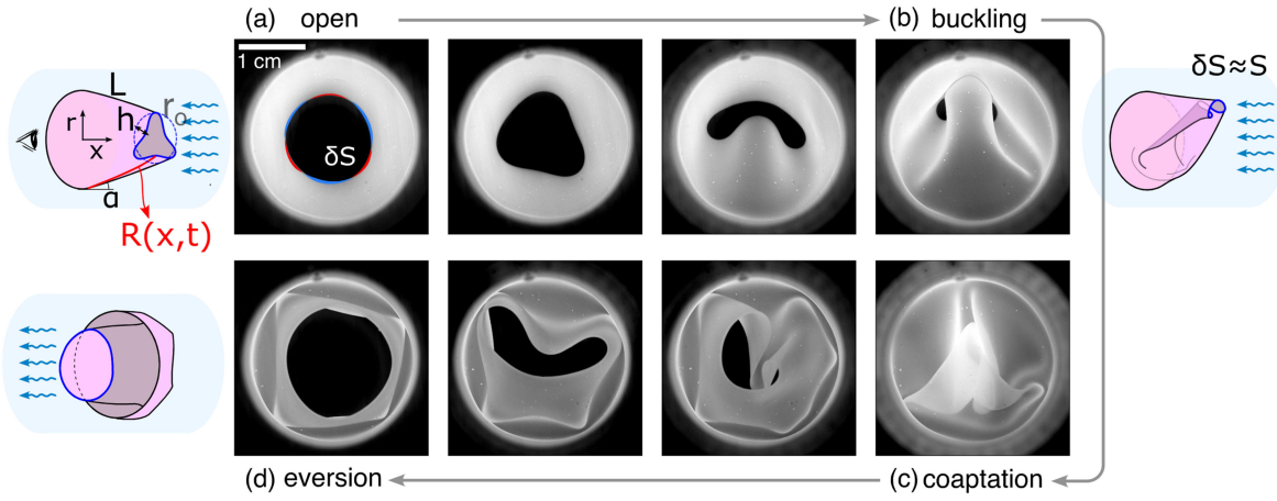
FIG. 2. High-speed images of a conical shell valve ( \alpha = 10^\circ ) buckling and everting under an impinging flow (ramping to an adverse pressure p \approx 100 Pa). The shell first oscillates (a) before buckling (b) to form a coaptation state (c). The shell eventually everts (d) at high p if not tethered. The schematics show the oscillating, buckled, and everted states of the cone. Coloring superimposed in (a): the area \delta S formed by the inward (blue) and outward (red) deformations of the orifice edge.
