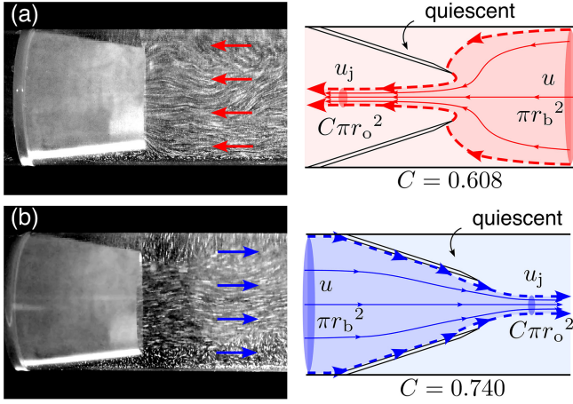
FIG. 7. The velocity field visualized by seeding particles for a flow against or along the direction of narrowing of a conical shell. Schematics: corresponding flow configurations giving rise to Eq. (A1). Dashed lines: velocity discontinuities (Helmholtz vortex sheets) that separate the jet (dark) and the quiescent regions (light).
