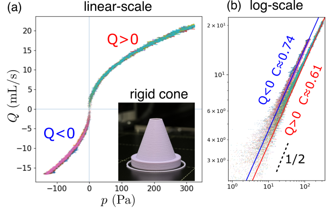
FIG. 8. (a) Pressure flow ( p - Q ) relation measured from a rigid cone of half-opening angle \alpha = 20^\circ (photograph). (b) Logarithmic scale of the same data as in (a). The effective coefficient C (0.74 or 0.61 for two flow directions) is extracted. Markers of different colors represent repeated experiments.
